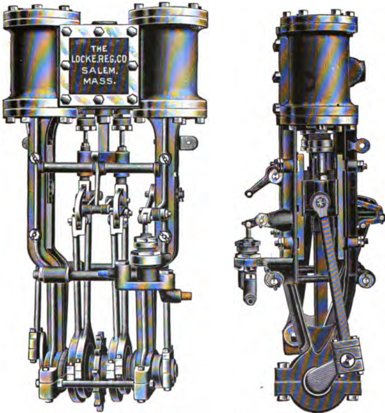
Figs. 256 and 257. —Front and Side Elevation of the "Locke" Steam Carriage Engine.
